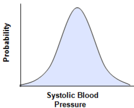
Figure 2. Gaussian distribution
